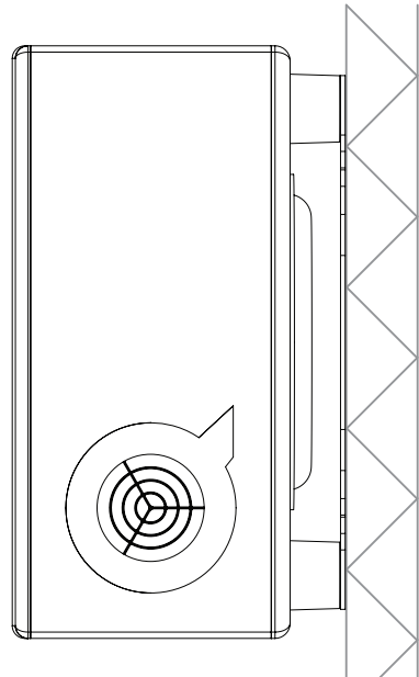
Example Wall Installation (using MPS10 kit)
